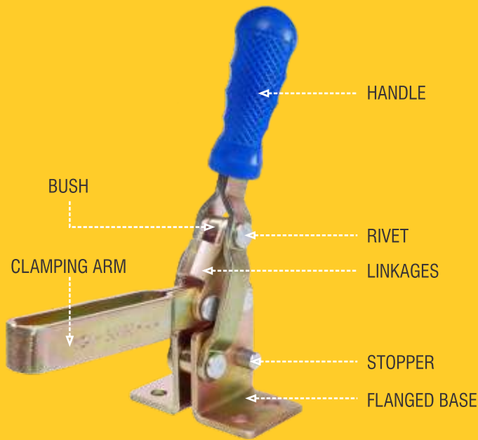
ELEMENTS OF TOGGLE CLAMP
